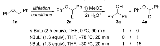
Scheme 2. \alpha -Lithiation of Benzyl Phenyl Ether 1a
